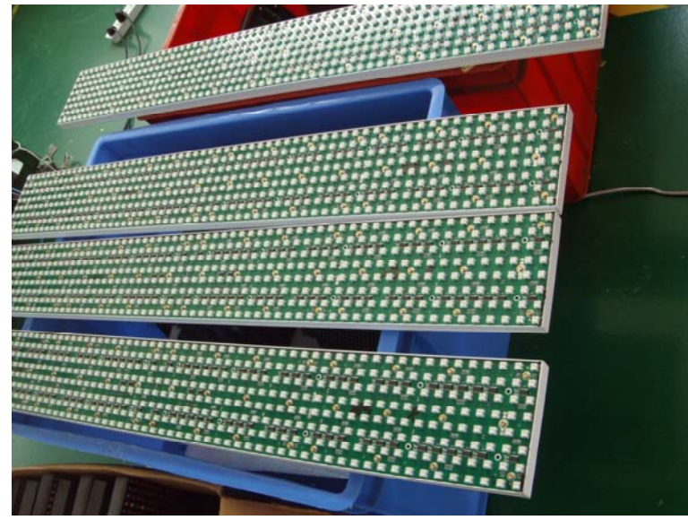
Before Potting compound
